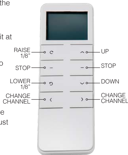
Figure 8: Multi-Channel Remote
